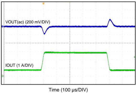
Figure 25. DCM Mode
